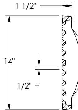
SECTION B-B
